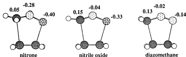
Figure 3. Atomic charges on the 1,3-dipolar unit in the RHF/3-21G TS (ref. [4] )
