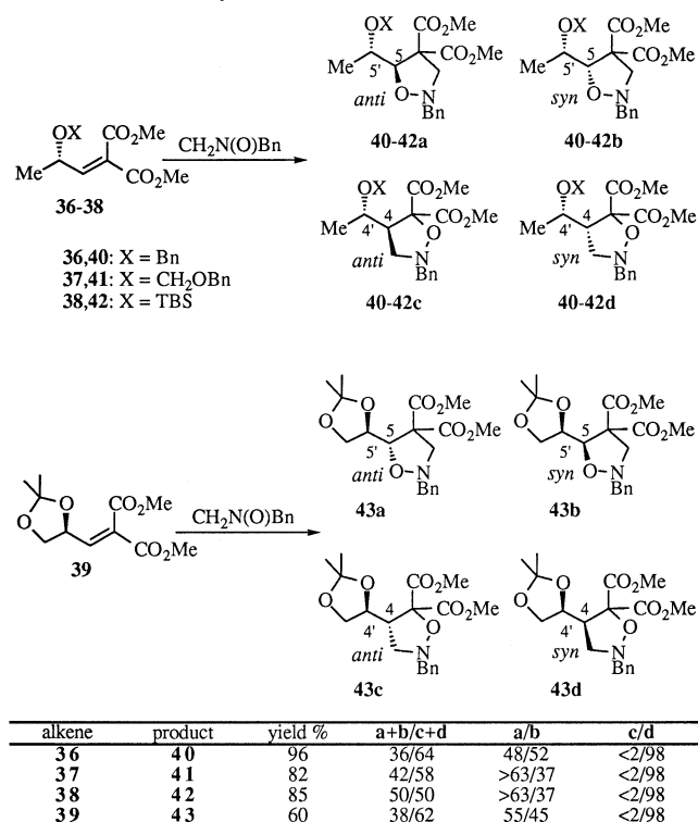
Scheme 4. Nitrone cycloadditions to 36–39
