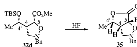
Scheme 3. Synthesis of bicyclic lactone 35
