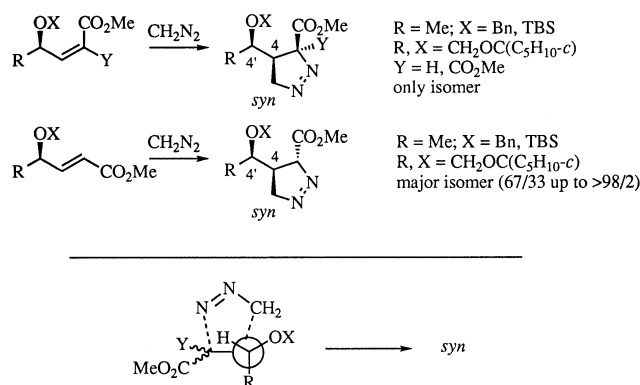
Figure 4. Diazomethane cycloaddition to \gamma -alkoxy- \alpha,\beta -unsaturated esters (ref. [6] )
