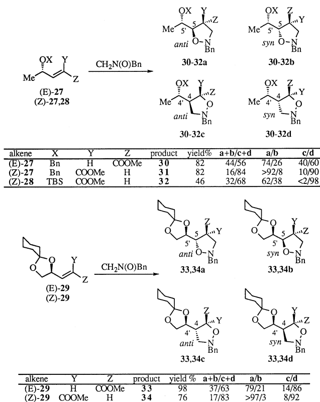
Scheme 2. Nitrone cycloaddition to ( E )- and ( Z )- 27–32
