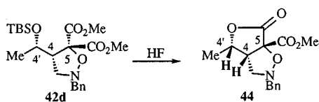
Scheme 5. Synthesis of bicyclic lactone 44
