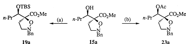
Scheme 1. Chemical correlation between compounds 15a , 19a , and 23a , and synthesis of compound 26a
